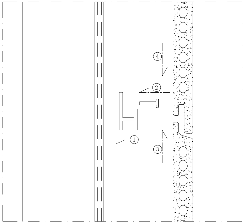
Installation of stone pendant 2D schematic diagram
