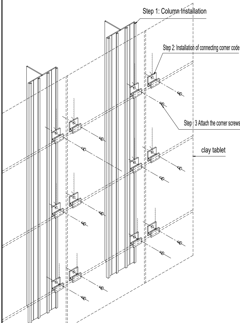
Installation of stone pendant steps
