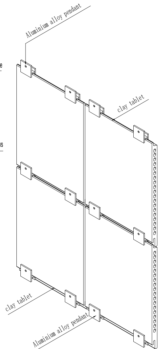
Installation diagram of pendant and stone panel
